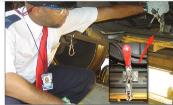
Figure 1-13 – Release folding stairs hold-down clamp
